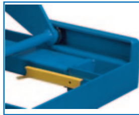
Rollers are entrapped in the base frame and platform for added stability
