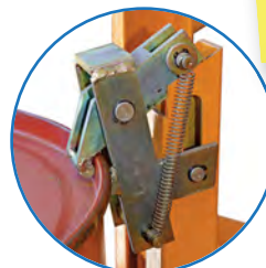
Spring loaded auto drum clamp
